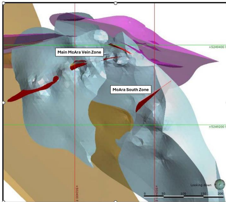
Figure 2: McAra Resource 3D Geological Model
